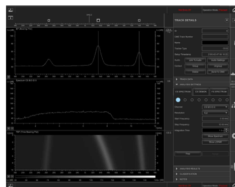
fig. 2: PILOS 2.0 HMI showing bearing, frequency and time bearing plots (night mode)
